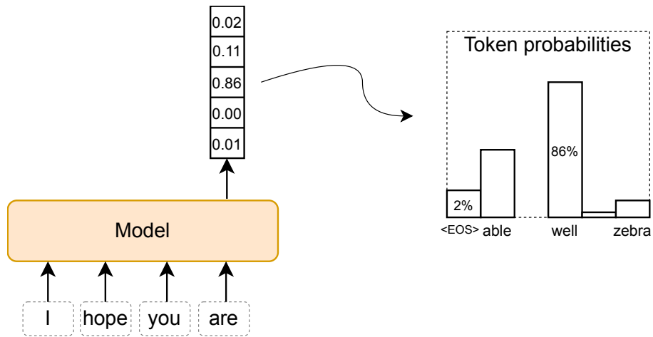
Figure 24: Probability distribution in next-token prediction
