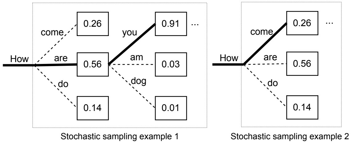
Figure 35: Stochastic sampling randomness
